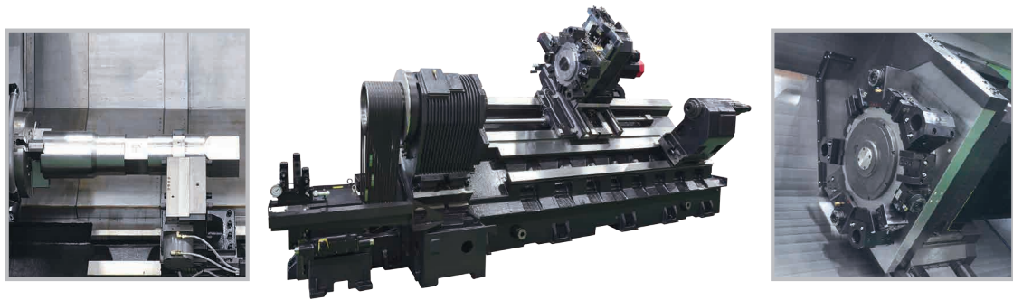
SL 4500LY 15~24" Y-Axis Horizontal Turning Center Offering High Precision with Vibration Preventing Low Center of Gravity and Minimal Thermal Displacement Design
