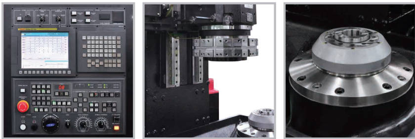
SLV 300 Vertical lathe developed for automatic process line of automobile and electric parts and maintain high accuracy in long-term machining process
