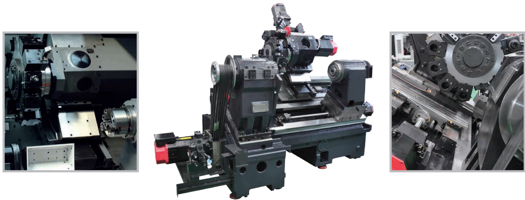
SL 2500SY Integrated machining operations in one set-up through Sub-spindle and Y-Axis
