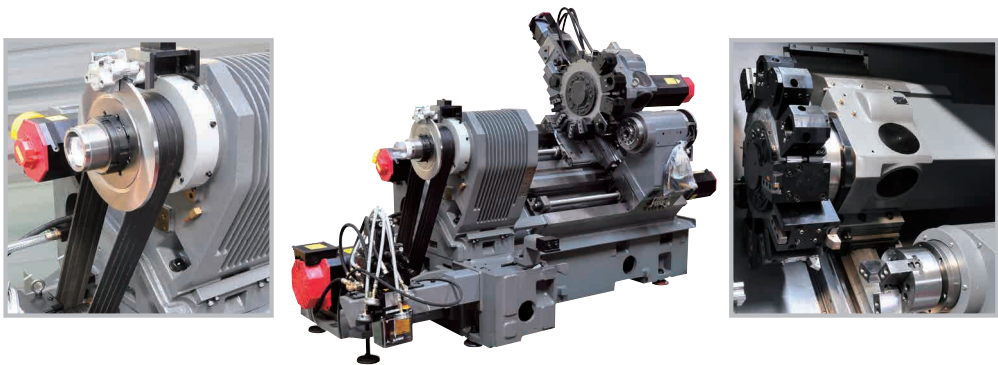
SL 2500MS Integrated machining operations in one set-up through Sub-spindle and Y-Axis
