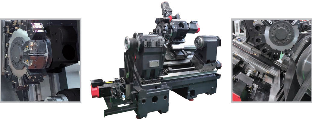
SL 2000SY Integrated machining operations in one set-up through Sub-spindle and Y-Axis
